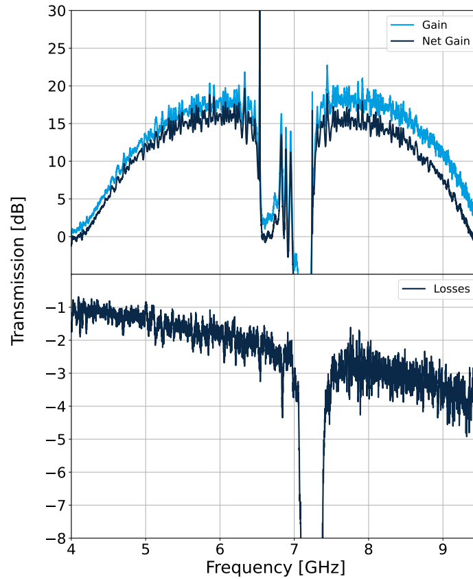
Figure 2: Top panel shows the gain (ON-OFF) and net gain (ON-lossless reference) of the TWPA. The pump parameters are (at the input of the TWPA): 6.889 GHz and -69.0 dBm. Bottom panel shows the electrical losses within the TWPA. The gap is centered at 7.25 GHz and is 0.39 GHz wide, the signal cannot propagate in the gap.
