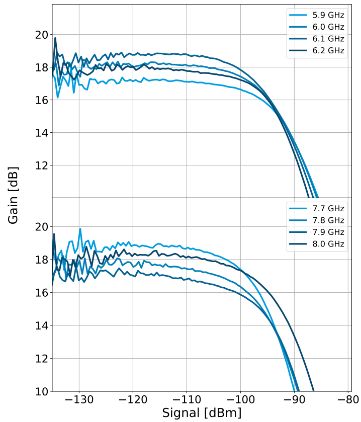
Figure 5: Graph of several saturation curves. The signal power corresponds to the signal at the input of the TWPA.
