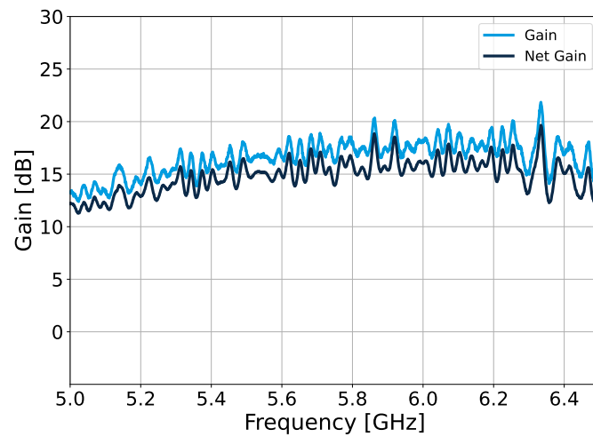
Figure 3: Zoom on the gain (ON-OFF) and net gain (ON-lossless reference) of the TWPA. The pump parameters are (at the input of the TWPA): 6.889 GHz and -69.0 dBm.
