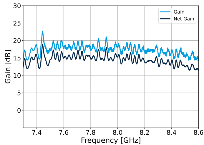
Figure 4: Zoom on the gain (ON-OFF) and net gain (ON-lossless reference) of the TWPA. The pump parameters are (at the input of the TWPA): 6.889 GHz and -69.0 dBm.
